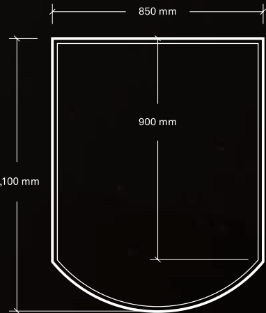
CURVED FRONT (Black & Opaque Only)
